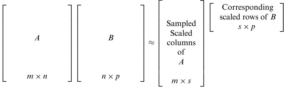
Figure 6.4: Approximate Matrix Multiplication using sampling.
