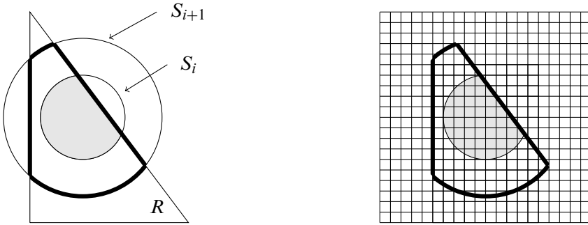
Figure 4.4: By sampling the area inside the dark line and determining the fraction of points in the shaded region we compute \frac{\text{Vol}(S_{i+1} \cap R)}{\text{Vol}(S_i \cap R)} . To sample, we create a grid and assign a probability of one to each grid point inside the dark lines and zero outside. Using Metropolis-Hasting edge probabilities, the stationary probability will be uniform for each point inside the the region, and we can sample points uniformly and determine the fraction within the shaded region.
