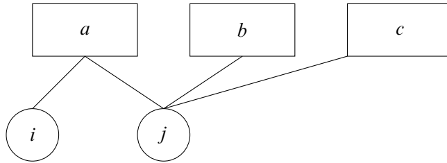
Figure 9.10: Warning propagation.
