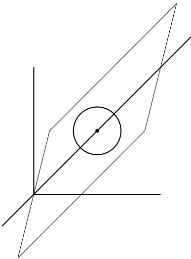
Figure 3.5: Best fit subspace to a spherical Gaussian.
