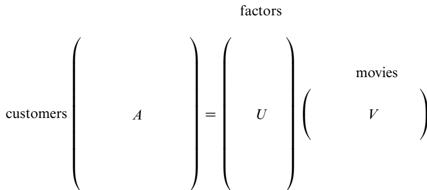
Figure 3.4: Customer-movie data
