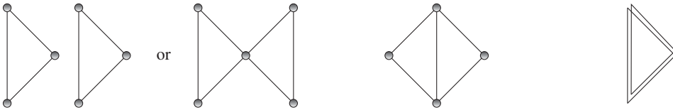
The two triangles of Part 1 are either disjoint or share at most one vertex
